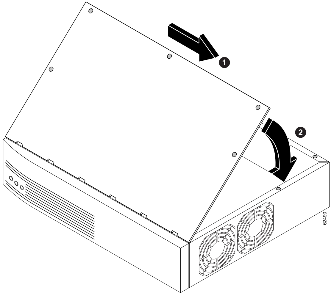
Figure 10 Replacing the Cisco 2691 Router Cover
